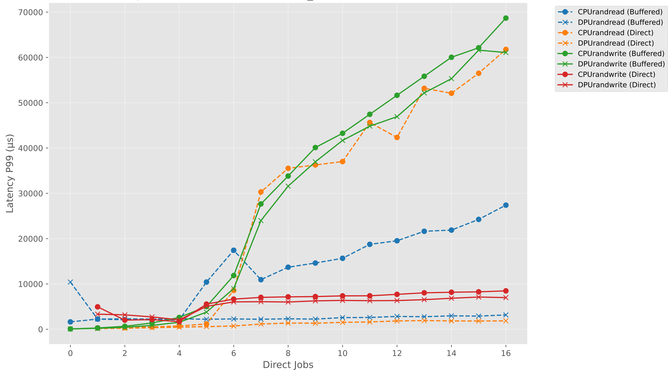
Latency P99 vs Direct Jobs (buffered1_directN) - RAND (CPU vs DPU)
